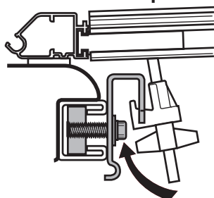
Cab Clamp
