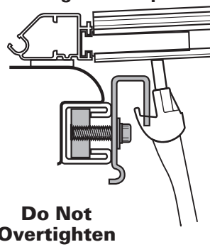
Tailgate Clamp
